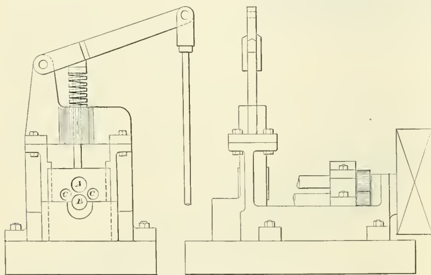
FLUE EXPANDING AND SWAGING MACHINE.
